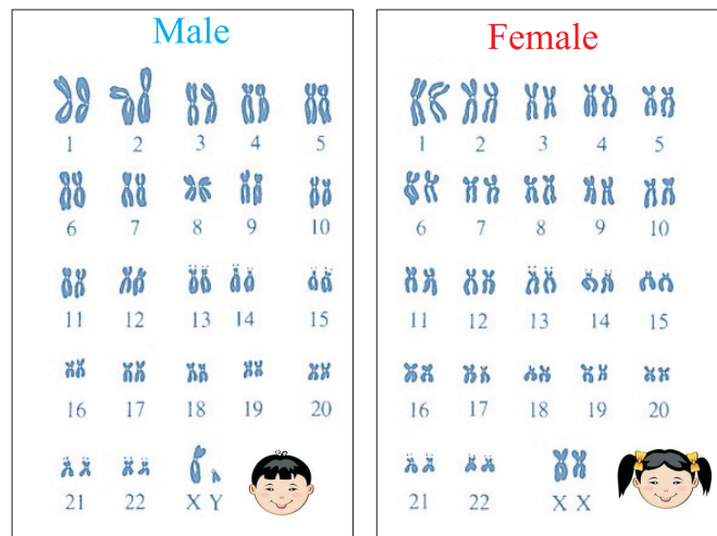
Fig 25.4 Human Chromosomes
