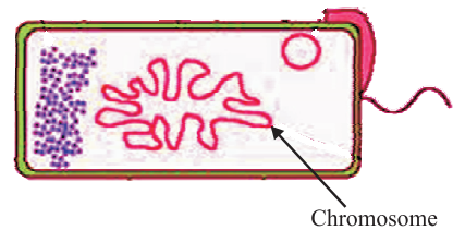
Fig. 25.3a Bacterial chromosome
