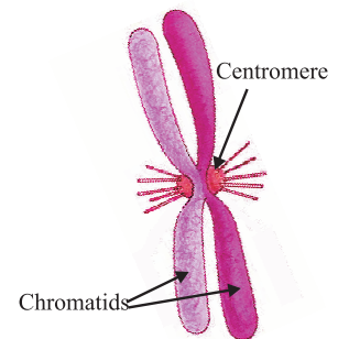
Fig. 25.3b Eukaryote chromosome
