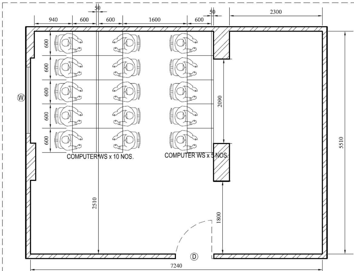
Furniture Layout Plan For Computer Room (NDLM LAB), Room No-105,1st Floor, A-31-NIOS, Noida
